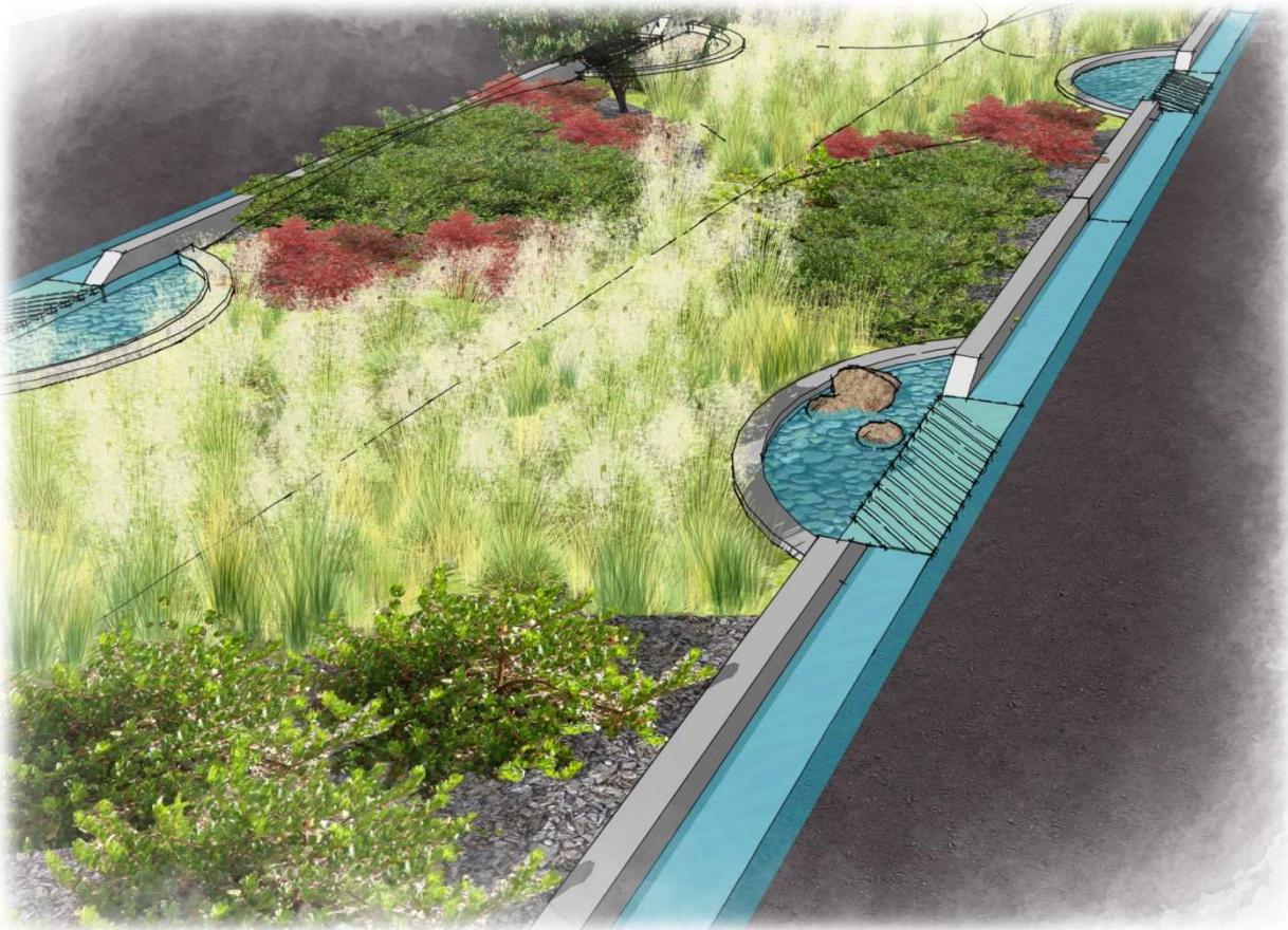
Illustration of LID median concept with street runoff directed to a depressed median with special curb and gutter inlets.
